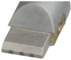
Diamond dresser Square 3 x 1,0 x 1,0 x 5 mm, Total bearing surface 3,0 mm 2 , r = 0,60 mm
