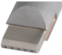
Diamond dresser Rhomboid 5 x 0,5 x 0,5 mm, Total bearing surface 1,25 mm 2 , r = 0,33 mm
