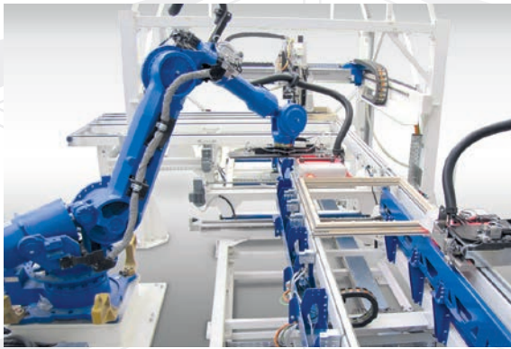
Window production plant
